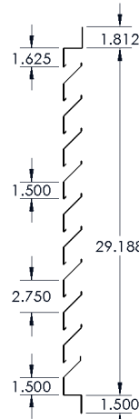
24" x 30" steel louver 157 sq. inches of free area 8 lbs. each/16 lbs. carton
