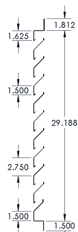
30" x 30" steel louver 202 sq. inches of free area 9 lbs. each/18 lbs. carton
