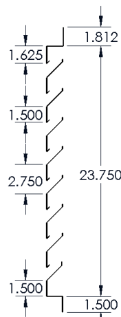
24" x 24" steel louver 126 sq. inches of free area 7 lbs. each/14 lbs. carton
