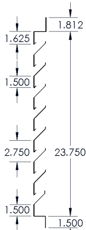
18" x 24" steel louver 90 sq. inches of free area 4 lbs. each/8 lbs. carton
